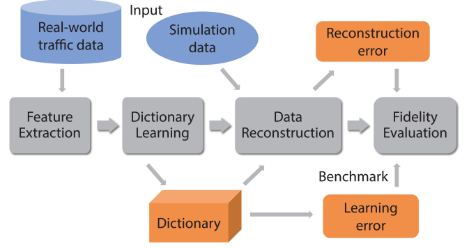
Fig. 2. The pipeline of our approach. The blue boxes show the input of the system, which contains real-world traffic dataset and simulation data to be evaluated.
