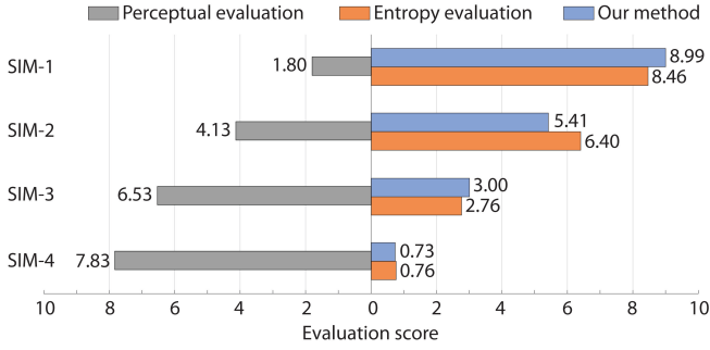
Fig. 6. The comparative user study results among the entropy-based scores (lower is better), our dictionary-based scores (lower is better), and the perceived similarity scores by participants (higher is better).
