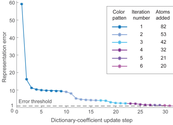
Fig. 7. The convergence of our adaptive dictionary learning algorithm. The curve segment in one color represents one iteration (i.e., one joint dictionary-coefficients optimization process after adaptively adding atoms to the dictionary). One point means the representation error after one dictionary-coefficient update step.
