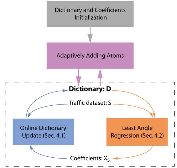
Fig. 3. Illustration of the joint dictionary-coefficients optimization process after adaptively adding atoms to the dictionary. The dictionary D is updated for the input real-world traffic flow dataset S via the online dictionary update algorithm. The least angle regression algorithm is employed to compute the coefficients X_S given the updated dictionary D . This process is repeated until convergence.
