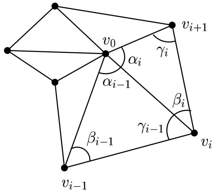
Figure Star-shaped polygon.
