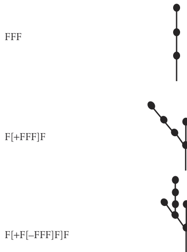
Figure 5.6 Some possible terminal strings
