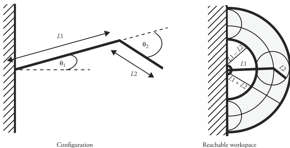
Figure 4.17 Simple linkage
