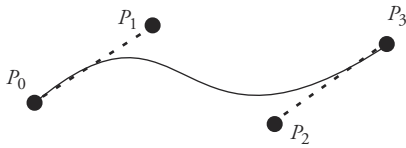
Figure B.34 Cubic Bezier curve segment
