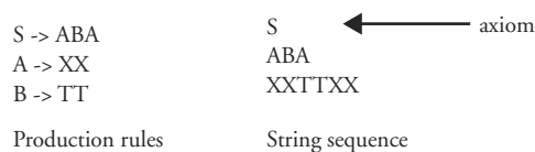
Figure 5.2 Simple DOL-system and the sequence of strings it generates
