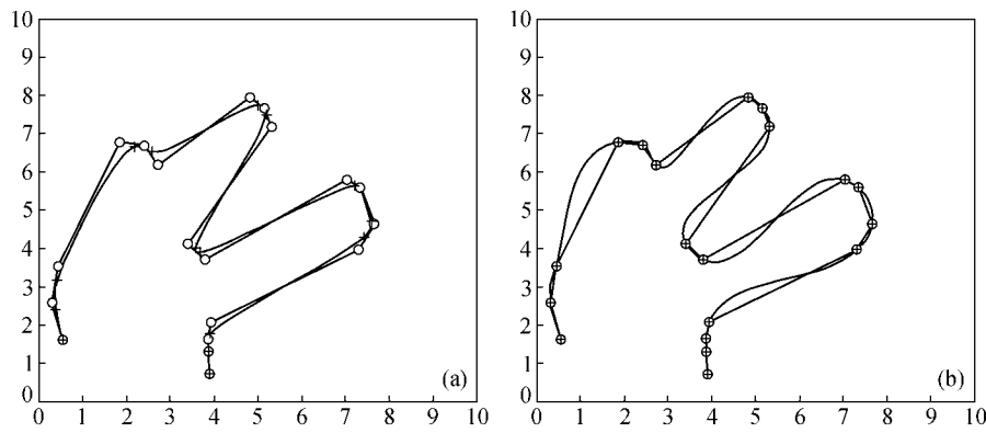
Fig. 4. Planar iterative non-uniform B-spline curve fitting a free curve. Left: The iterative time is 0, the error is 4.222137\text{e-}001 ; Right: the iterative time is 30, the error is 7.073353\text{e-}005 .
