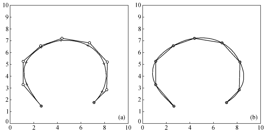
Fig. 5. The convexity-preserving property of the planar iterative non-uniform B-spline curve. Left: The iterative time is 0, the error is 3.700325\text{e-}001 ; Right: the iterative curve is convexity-preserving after 30 times iteration, the error is 8.389196\text{e-}008 .
