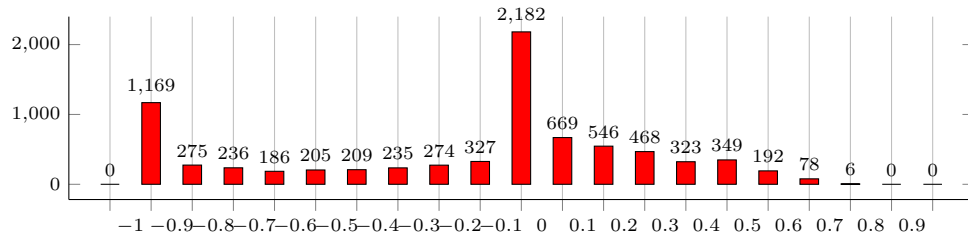
Figure 4: Distribution of minimum scaled Jacobian.
