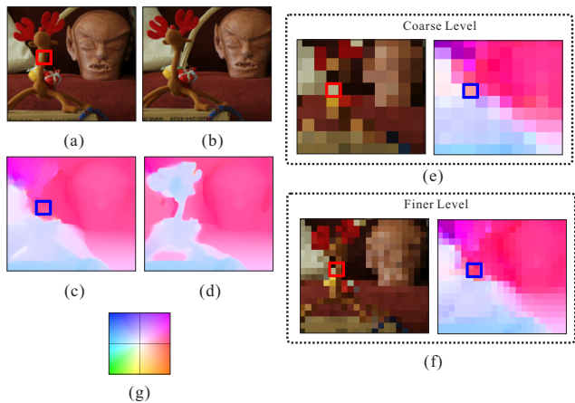
Figure 1. Motion detail preserving problem. (a)-(b) Two input patches. (c) Flow estimate using the coarse-to-fine variational setting. (d) Our flow estimate. (e)-(f) Two consecutive levels in the pyramid. Flow maps are visualized using the color code in (g).
