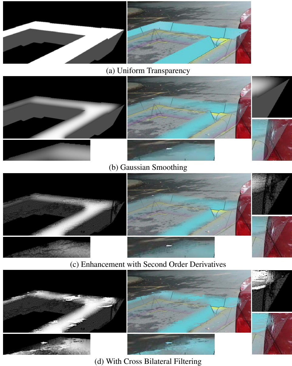
Figure 3.4: Mask for color blending. From upper row to bottom one: uniform transparency, smoothing the edge inside, with modulation by image second order derivative, with using cross bilateral filtering. Note that modulation by curvature tends to preserve discontinuities and that cross bilateral filtering tends to preserve uniform regions (like the upper-left dark mark on the road).
